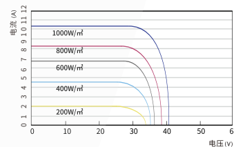
LNSK-335M/I-V
